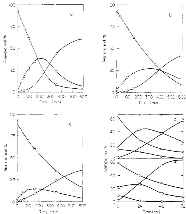
Figure 1. Composition plots for the reactions of 1 and 2 : (a) 1 , 50 °C, 2 M in CD 3 CN; (b) 1 , 50 °C, 1 M in CD 3 CN; (c) 1 , 50 °C, 2 M in toluene- d 8 ; (d) 2 , room temperature, 0.5 M in CD 3 CN; (e) 2 , room temperature, 0.5 M in toluene- d 8 . (Δ) Diazo compound; (O) E,E azine; (□) E,Z azine; (◇) Z,Z azine.
