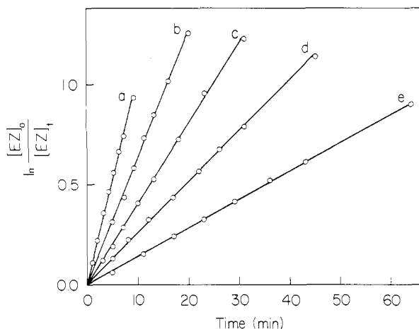
Figure 2. Kinetic plots for the thermal isomerization of ( E,Z )-4 at various temperatures: (a) 75 °C; (b) 70 °C; (c) 65 °C; (d) 60 °C; (e) 55 °C.
